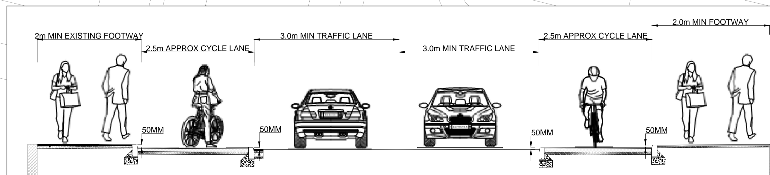
TYPICAL SECTION THROUGH SOUTH CITY WAY TIERED CYCLE PROVISION
